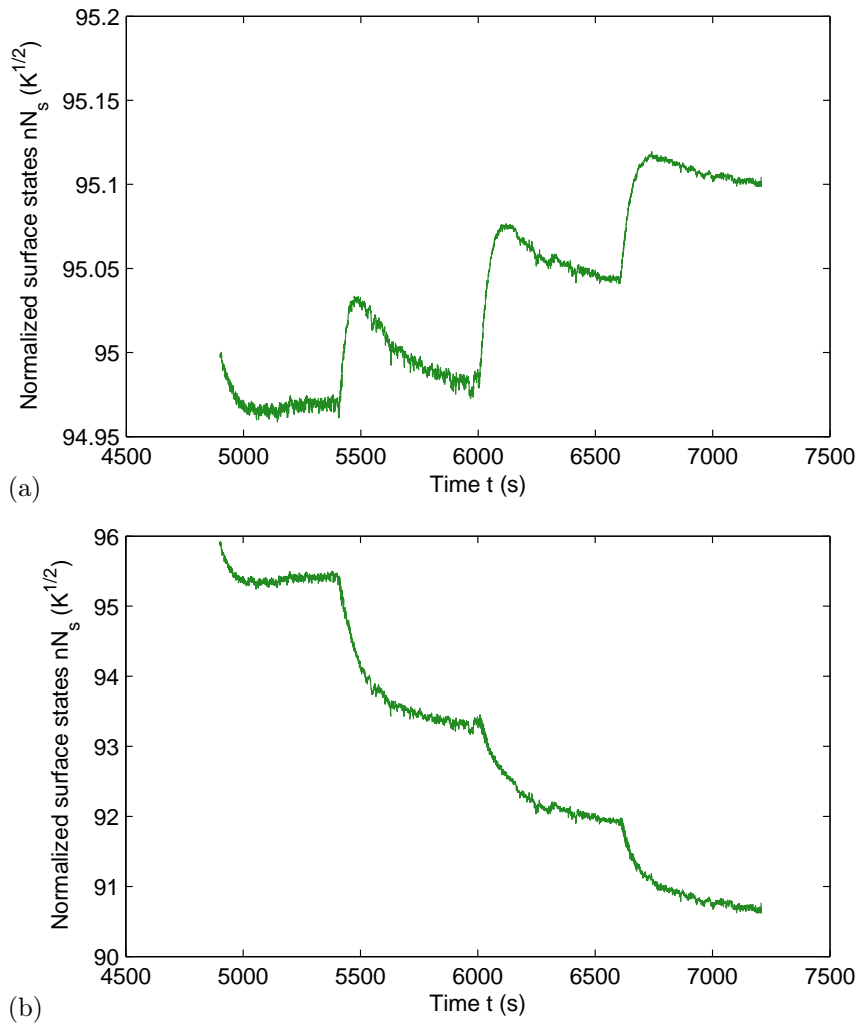
Figure 6.3: Plot of the normalized surface state density nN_s for the completely (a) and partly depleted case (b).
