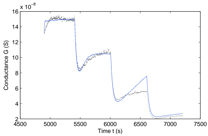
Figure 6.5: Simulated conductance G for computed nN_s values from parameter set in Table 6.2 vs. measured conductance values.
